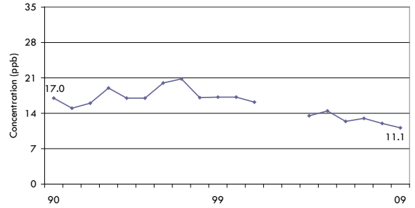
Figure D7 NO 2 Annual Mean at Oakville
