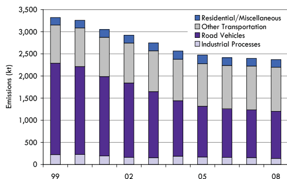
Figure 4.6 Ontario Carbon Monoxide Emission Trend (1999-2008)
