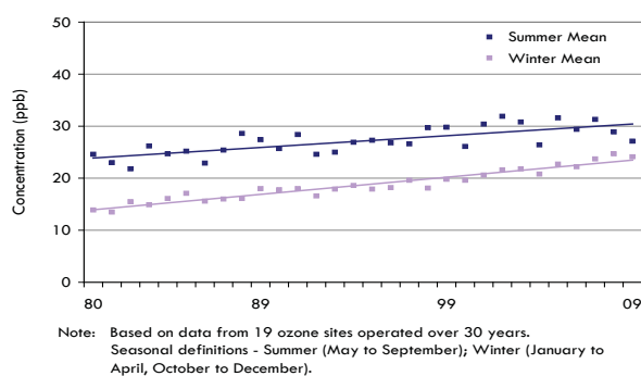
Figure 2.5 Trend of Ozone Seasonal Means at Sites Across Ontario (1980-2009)
