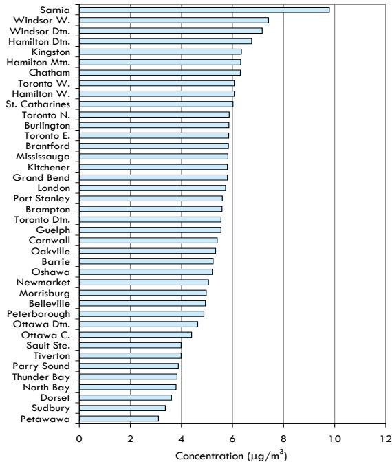
Figure 3.2 Annual Mean PM 2.5 Concentrations Across Ontario (2009)
