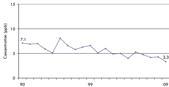
Figure F6 SO 2 Annual Mean at Hamilton Downtown
