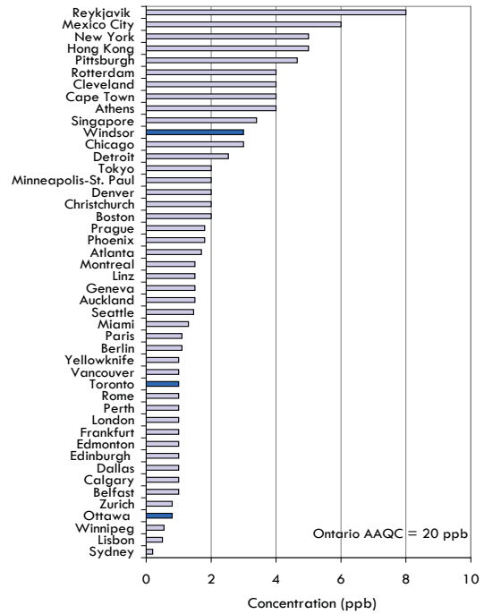
Figure 6.6 Sulphur Dioxide Annual Means for Selected Cities World-wide (2009)
