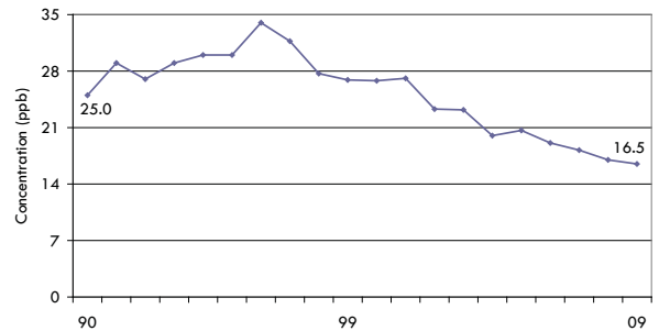
Figure D8 NO 2 Annual Mean at Toronto Downtown
