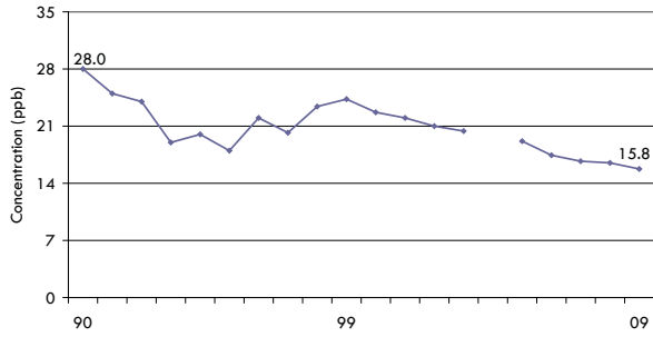
Figure D9 NO 2 Annual Mean at Toronto North
