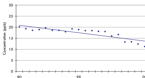
Figure 4.1 Trend of Nitrogen Dioxide Annual Means in Ontario (1990-2009)
