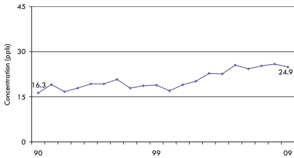
Figure C2 Ozone Annual Mean at Windsor West
