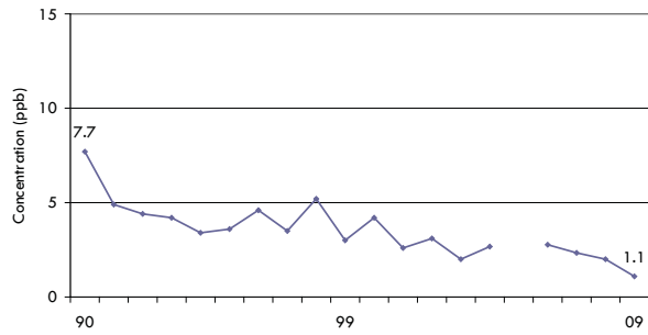
Figure F9 SO 2 Annual Mean at Sudbury
