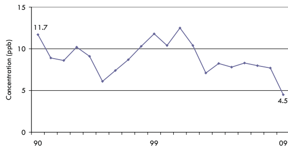
Figure F4 SO 2 Annual Mean at Sarnia
