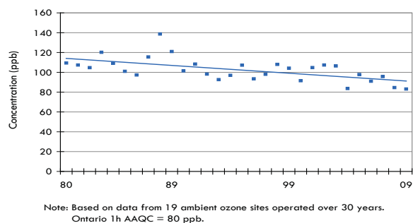
Figure 2.4 Trend of Ozone One-Hour Maximum Concentrations in Ontario (1980-2009)
