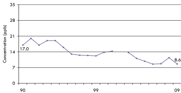
Figure D12 NO 2 Annual Mean at Ottawa Downtown
