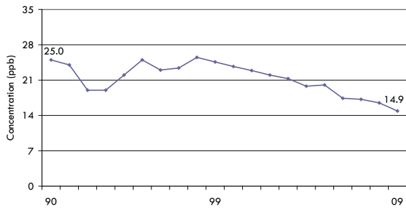
Figure D10 NO 2 Annual Mean at Toronto East
