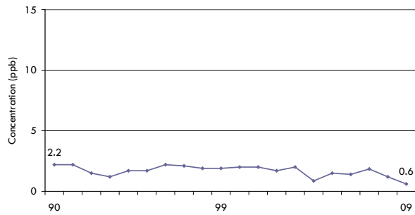
Figure F10 SO 2 Annual Mean at Sault Ste. Marie
