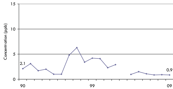
Figure F8 SO 2 Annual Mean at Ottawa Downtown
