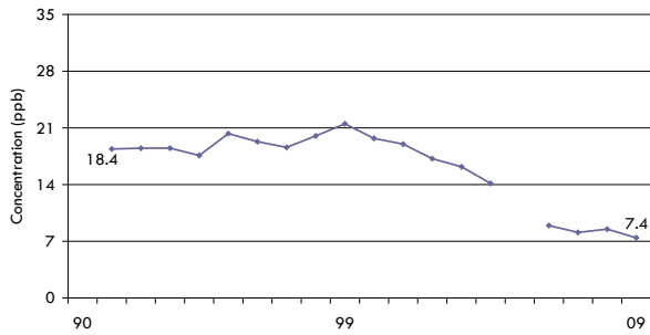
Figure D11 NO 2 Annual Mean at Oshawa
