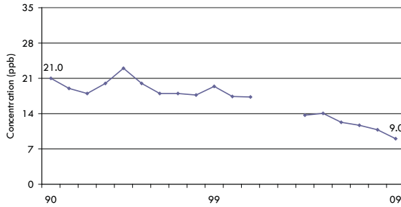
Figure D2 NO 2 Annual Mean at London
