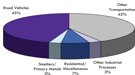
Figure 4.4 Ontario Carbon Monoxide Emissions by Sector (Emissions from Point/Area/Transportation Sources, 2008 Estimates)
