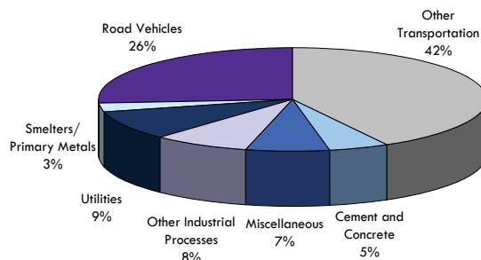
Figure 2.2 Ontario Nitrogen Oxides Emissions by Sector (Emissions from Point/Area/Transportation Sources, 2008 Estimates)
