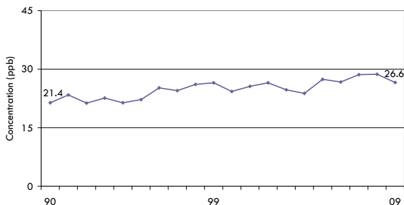
Figure C4 Ozone Annual Mean at Sarnia
