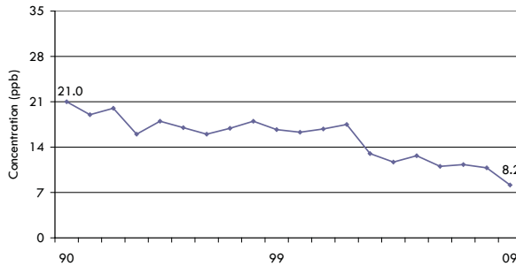
Figure D3 NO 2 Annual Mean at Sarnia
