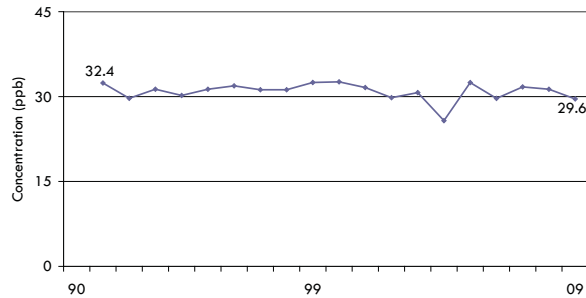
Figure C5 Ozone Annual Mean at Grand Bend
