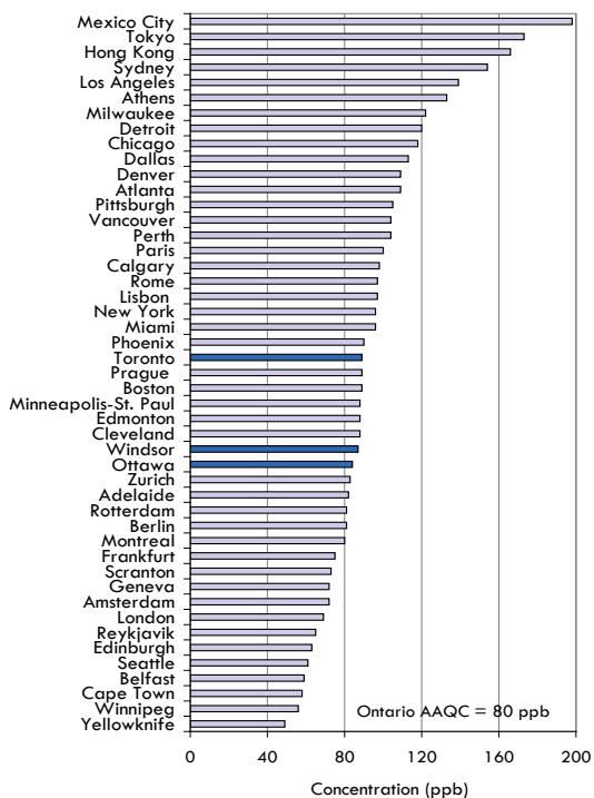
Figure 6.2 Ozone One-Hour Maximum Concentrations for Selected Cities World-wide (2009)
