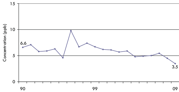
Figure F1 SO 2 Annual Mean at Windsor Downtown
