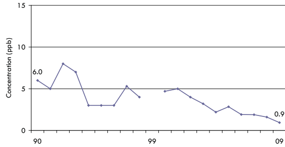
Figure F7 SO 2 Annual Mean at Toronto Downtown
