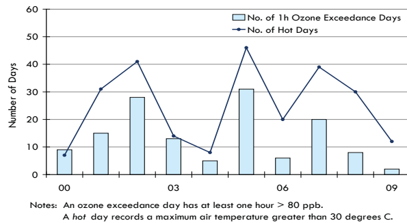
Figure 2.7 Trend of Ozone Exceedance Days and Hot Days at Windsor Downtown (2000-2009)
