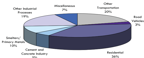
Figure 3.1 Ontario PM_{2.5} Emissions by Sector (Emissions from Point/Area/Transportation Sources, 2008 Estimates)
