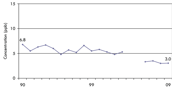
Figure F5 SO 2 Annual Mean at Hamilton Mountain
