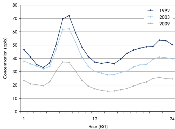
Figure 4.3 Diurnal Trend of NO x at Toronto East (1992, 2003, 2009)
