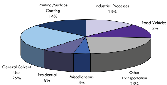
Figure 2.1 Ontario Volatile Organic Compounds Emissions by Sector (Emissions from Point/Area/Transportation Sources, 2008 Estimates)
