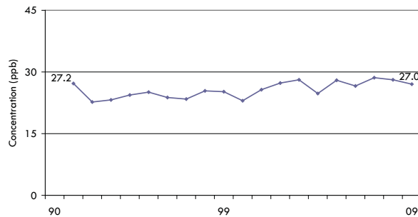
Figure C7 Ozone Annual Mean at Kitchener
