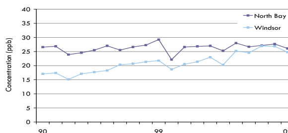
Figure 2.6 Ozone Annual Mean Concentrations at Windsor Downtown and North Bay (1990-2009)
