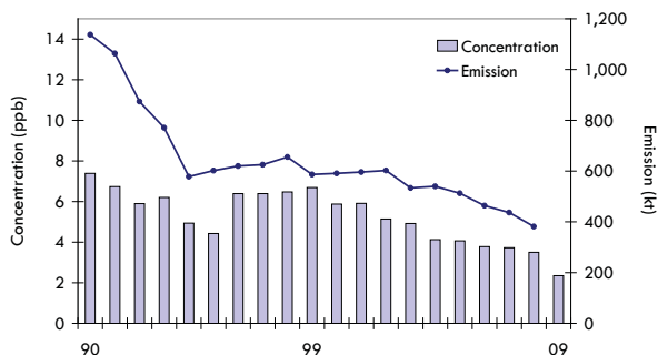
Figure 4.8 Ontario Sulphur Dioxide Annual Mean Concentrations and Emissions Trend (1990-2009)
