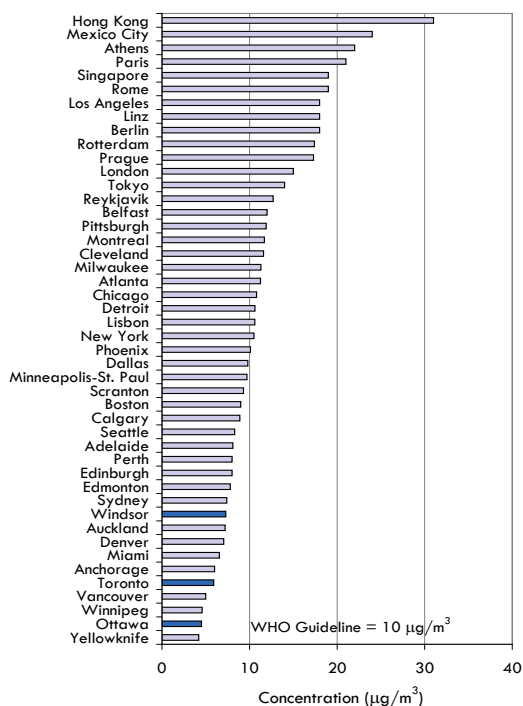
Figure 6.3 PM 2.5 Annual Means for Selected Cities World-wide (2009)
