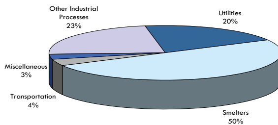
Figure 4.7 Ontario Sulphur Dioxide Emissions by Sector (Emissions from Point/Area/Transportation Sources, 2008 Estimates)
