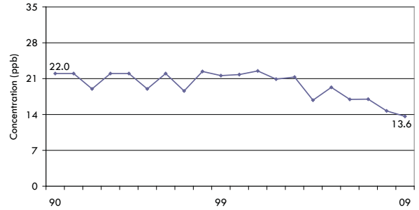
Figure D5 NO 2 Annual Mean at Hamilton Downtown
