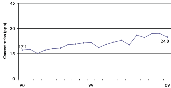
Figure C1 Ozone Annual Mean at Windsor Downtown
