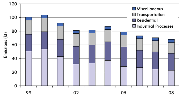
Figure 3.4 Ontario PM 2.5 Emission Trend (1999-2008)
