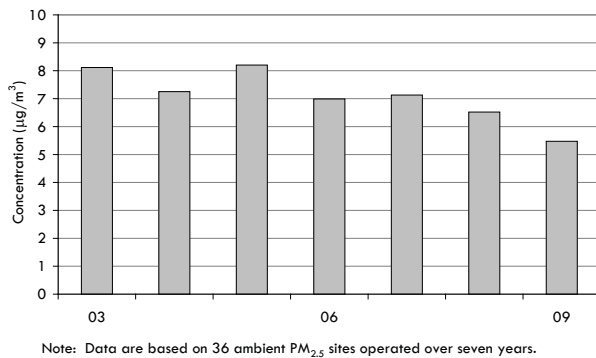
Figure 3.3 Provincial Annual Composite Mean PM 2.5 Concentrations (2003-2009)
