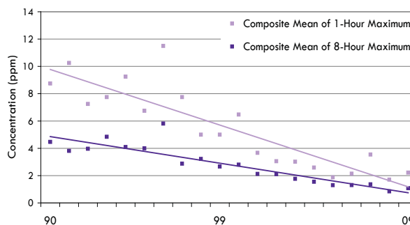
Figure 4.5 Trends of Carbon Monoxide One-Hour and Eight-Hour Maximums in Ontario (1990-2009)
