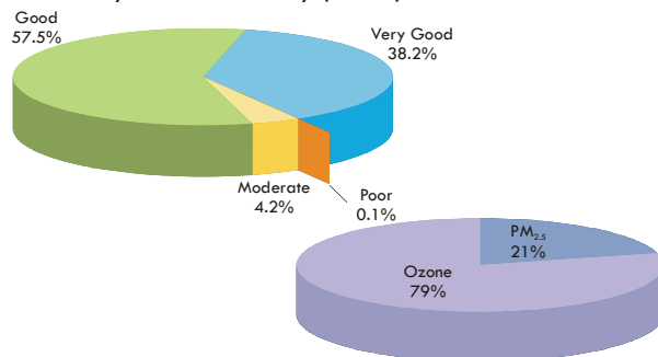
Figure 5.2 Air Quality Index Summary (2009)
