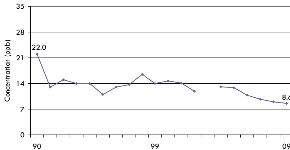
Figure D4 NO 2 Annual Mean at Kitchener
