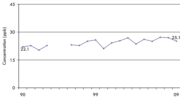
Figure C3 Ozone Annual Mean at London
