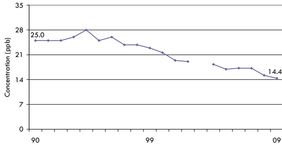
Figure D1 NO 2 Annual Mean at Windsor Downtown
