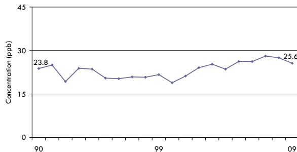
Figure C8 Ozone Annual Mean at St. Catharines
