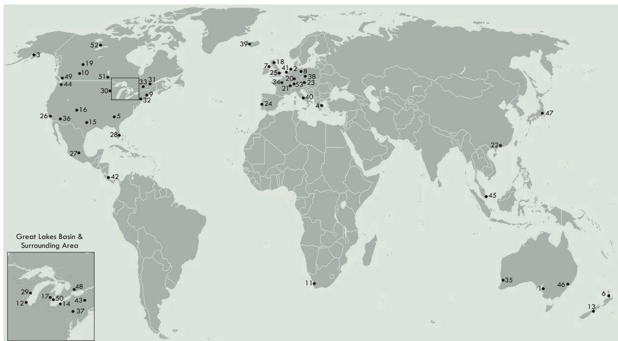
Figure 6.1 Selected Cities Around the World Used for 2009 Air Quality Comparison
