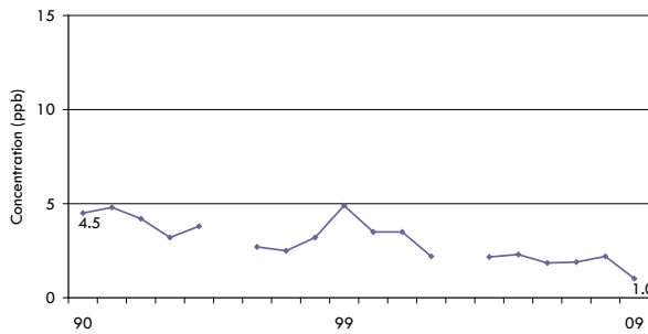
Figure F3 SO 2 Annual Mean at London
