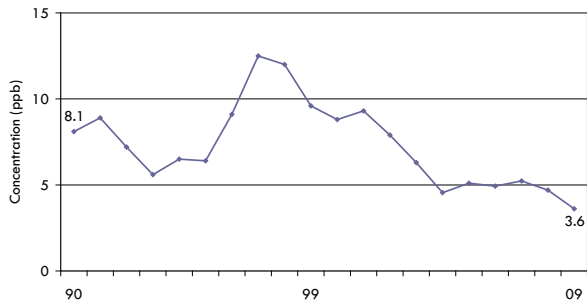
Figure F2 SO 2 Annual Mean at Windsor West
