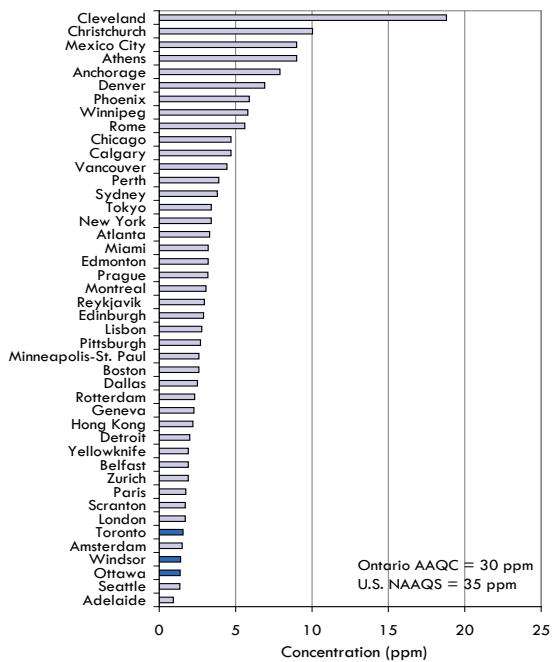
Figure 6.5 Carbon Monoxide One-Hour Maximum Concentrations for Selected Cities World-wide (2009)
