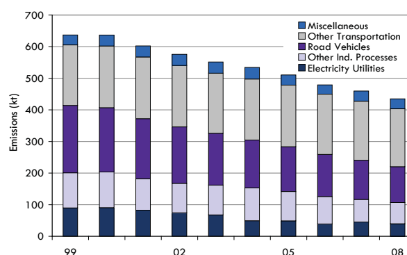
Figure 4.2 Ontario Nitrogen Oxides Emission Trend (1999-2008)
