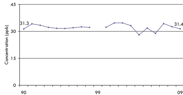
Figure C6 Ozone Annual Mean at Tiverton
