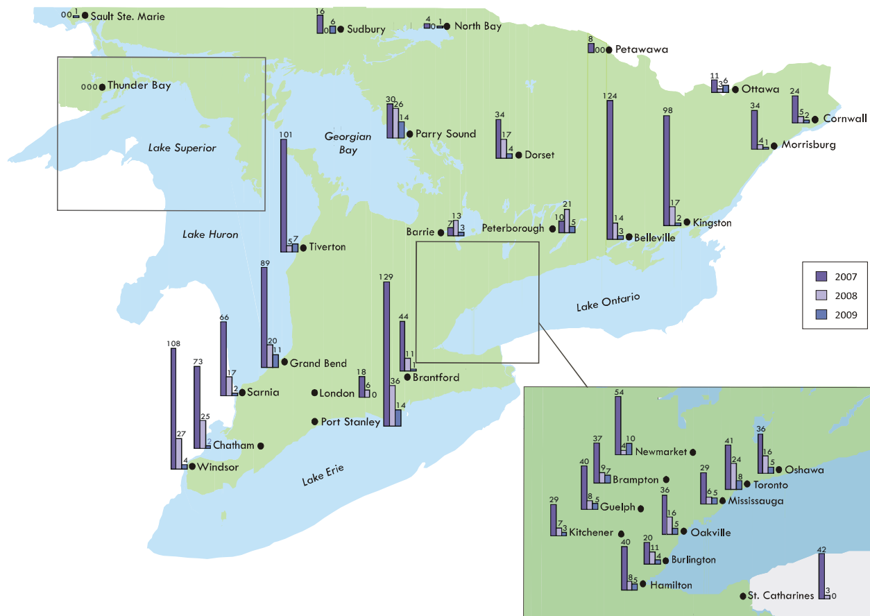
Figure 2.3 Geographical Distribution of Number of One-Hour Ozone Exceedances Across Ontario (2007, 2008, 2009)
