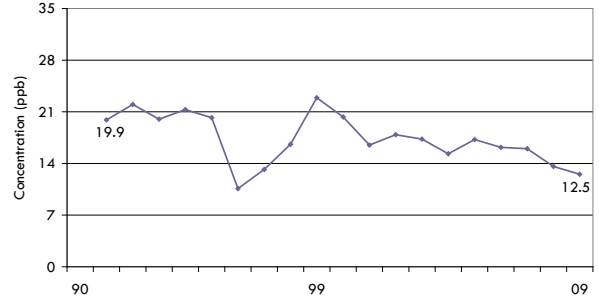
Figure D6 NO 2 Annual Mean at Burlington
